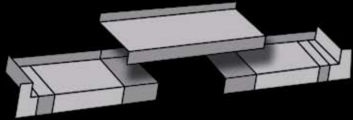
Telescopes for adjustability during installation
